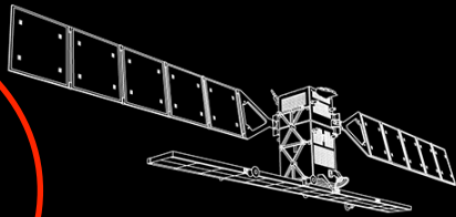
sentinel-1
