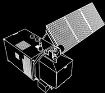
sentinel-2
